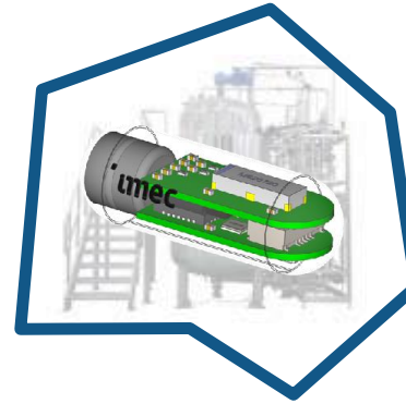
PATcube sensor
